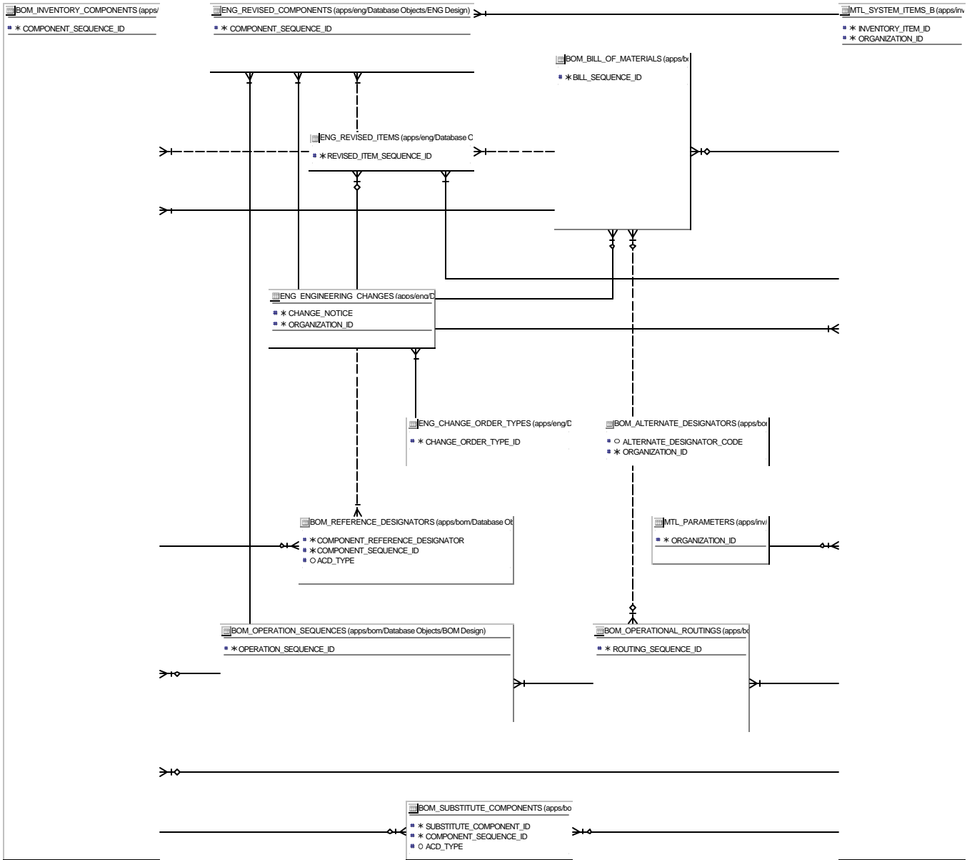
Diagram : R115 ENG SUMMARY DB DIAGRAM Modified : 22 February 1999 12:46:44 Application System : apps/bom/Database Objects/BOM Design
