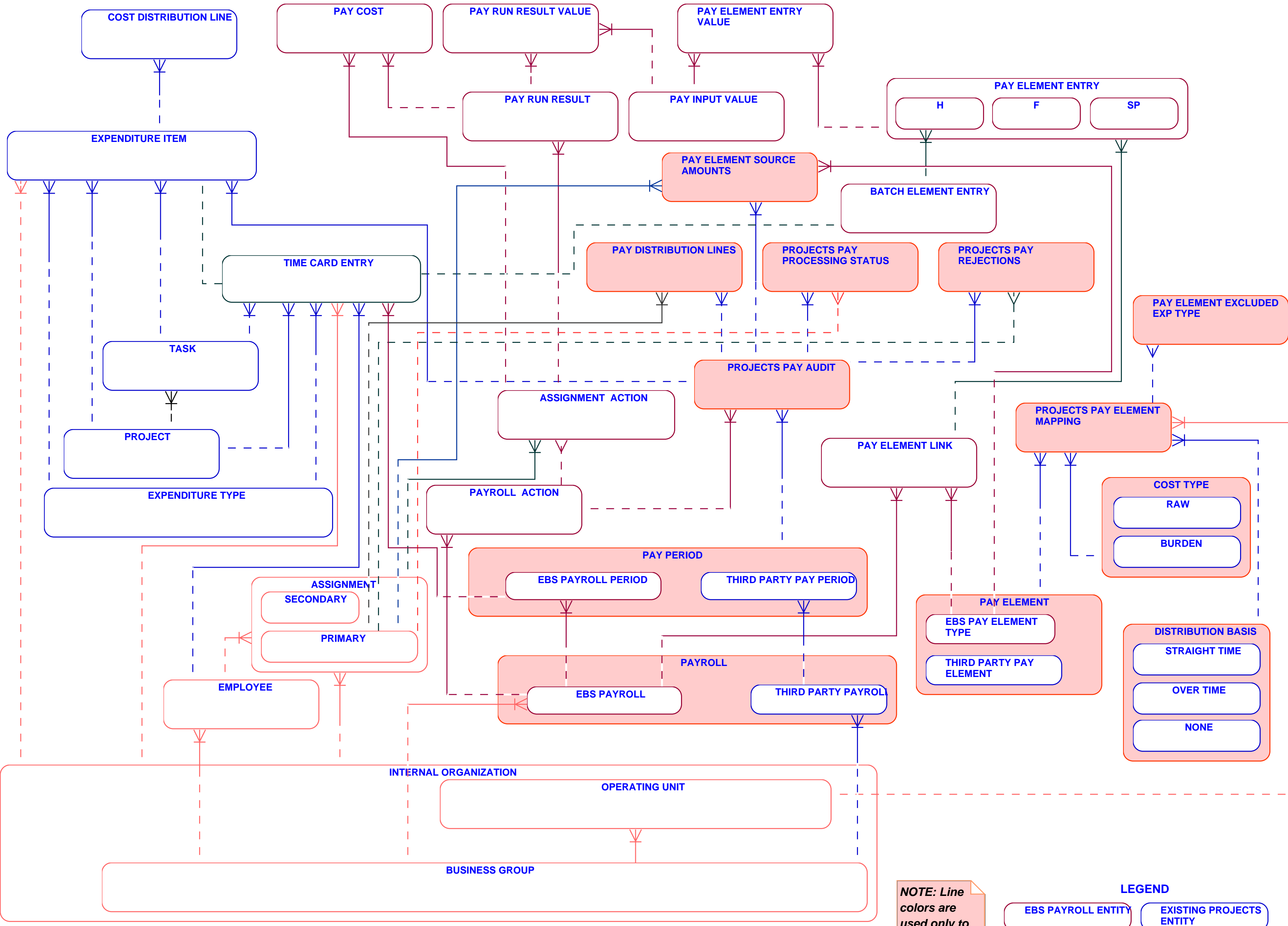
ER Diagram for Payroll-Projects Integration
